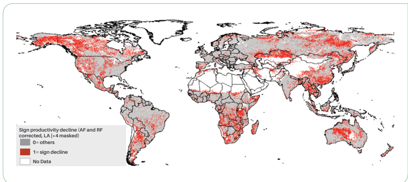
Figure 4.1 Areas of human-induced biomass productivity decline over the period 1982–2006 (red area) with significant trend ( p < 0.1 , trend magnitude >10\% of baseline year/25 years), rainfall and atmospheric effects corrected. Source: Le et al. (2016).
